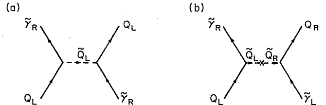
FIG. 1. Exchange of a scalar quark mediates a quark-photino interaction. Part (a), which is always present, gives a spin dependent force; (b), which is present only if there is strong mixing of left- and right-handed scalar quarks, gives a coherent interaction.
