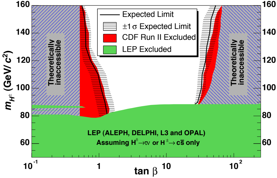
Figure 11: Summary of the 95% C.L. exclusions in the (m_{H^\pm}, \tan\beta) plane obtained by LEP [158] and CDF [177]. The benchmark scenario parameters used to interpret the CDF results are very close to those of the m_h^{\max} scenario, and m_t is assumed to be 175 GeV. The full lines indicate the median limits expected in the absence of a H^\pm signal, and the horizontal hatching represents the \pm 1\sigma bands about this expectation.
