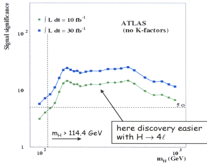
Figure 3. Higgs discovery potential for one of the LHC detectors, as a function of the Higgs mass, for two values of the integrated luminosity.
