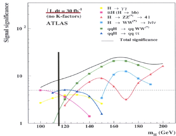
Figure 4. Higgs discovery potential in the low mass region. In particular for the lowest masses the combination of various decay channels is required in order to optimize the signal.
